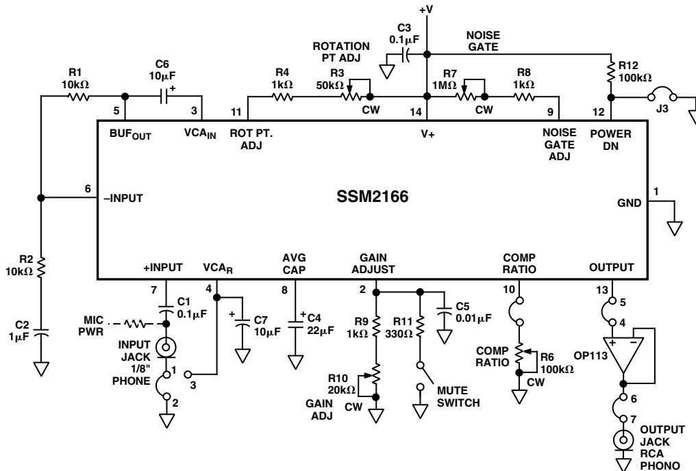
Figure 12. Evaluation Board
